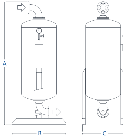
Flange connection
